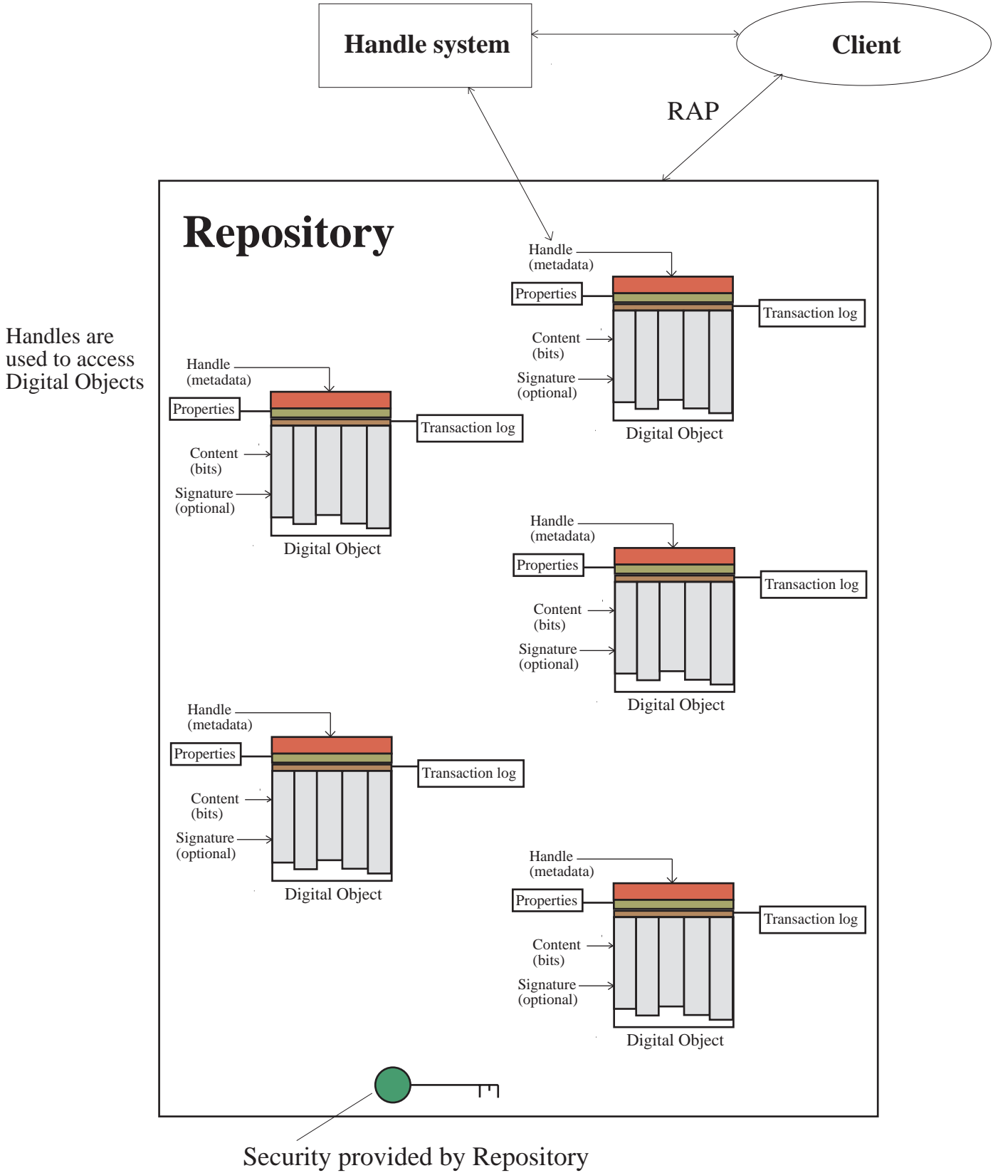
Figure 11.1 Digital objects, handles and repositories.
